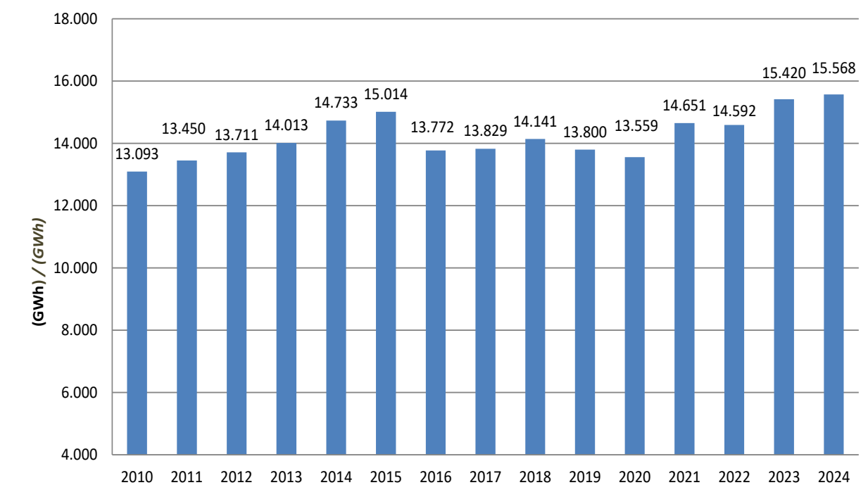
Graph 8.2.1 - Evolution of the Final Consumption of Electric Energy in Espírito Santo * - Values in GWh
