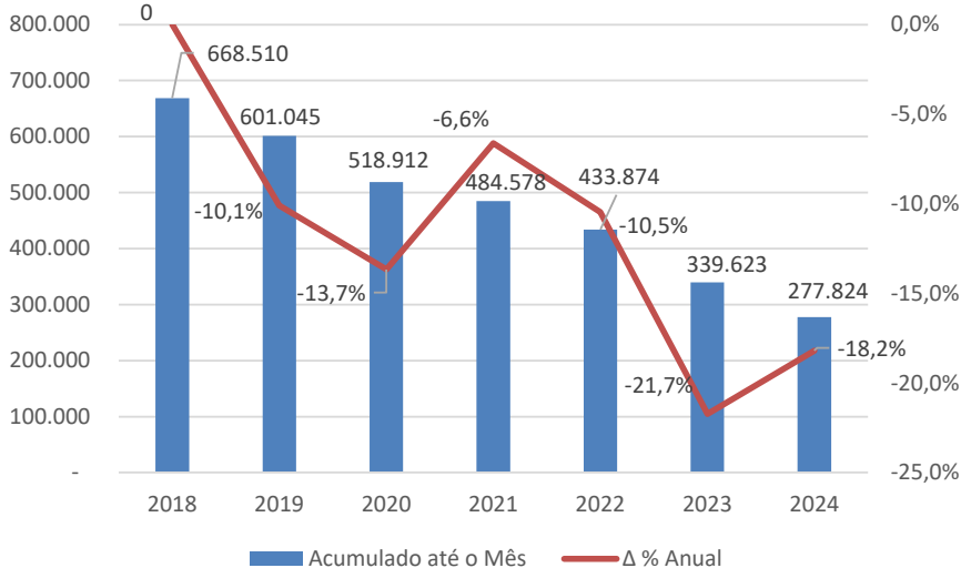
Consumo Industrial (MWh)
