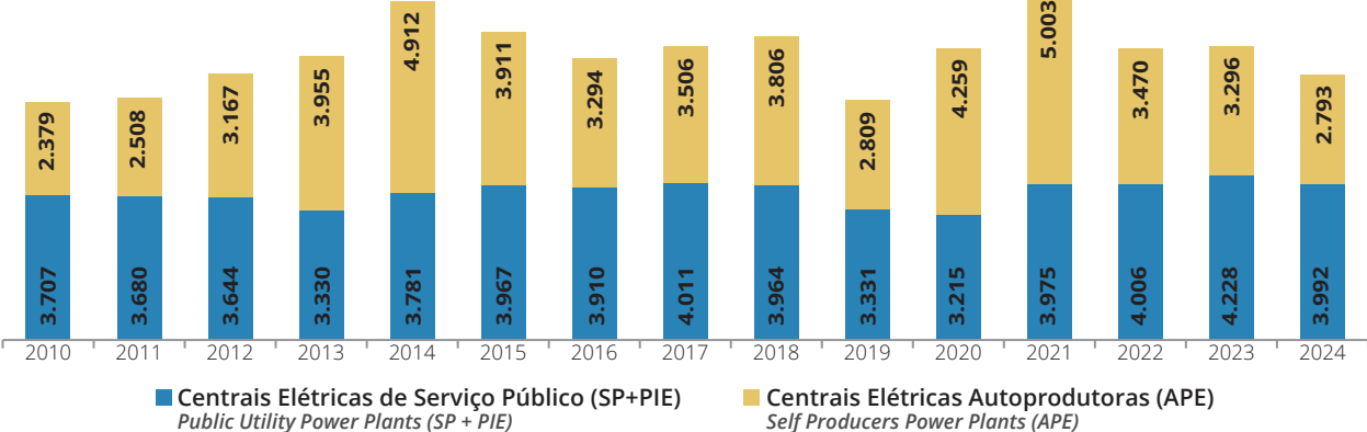
Graph 8.1.1 - Evolution of Electric Power Generation - Self-production X Public Service in the ES - Values in thousand toe
