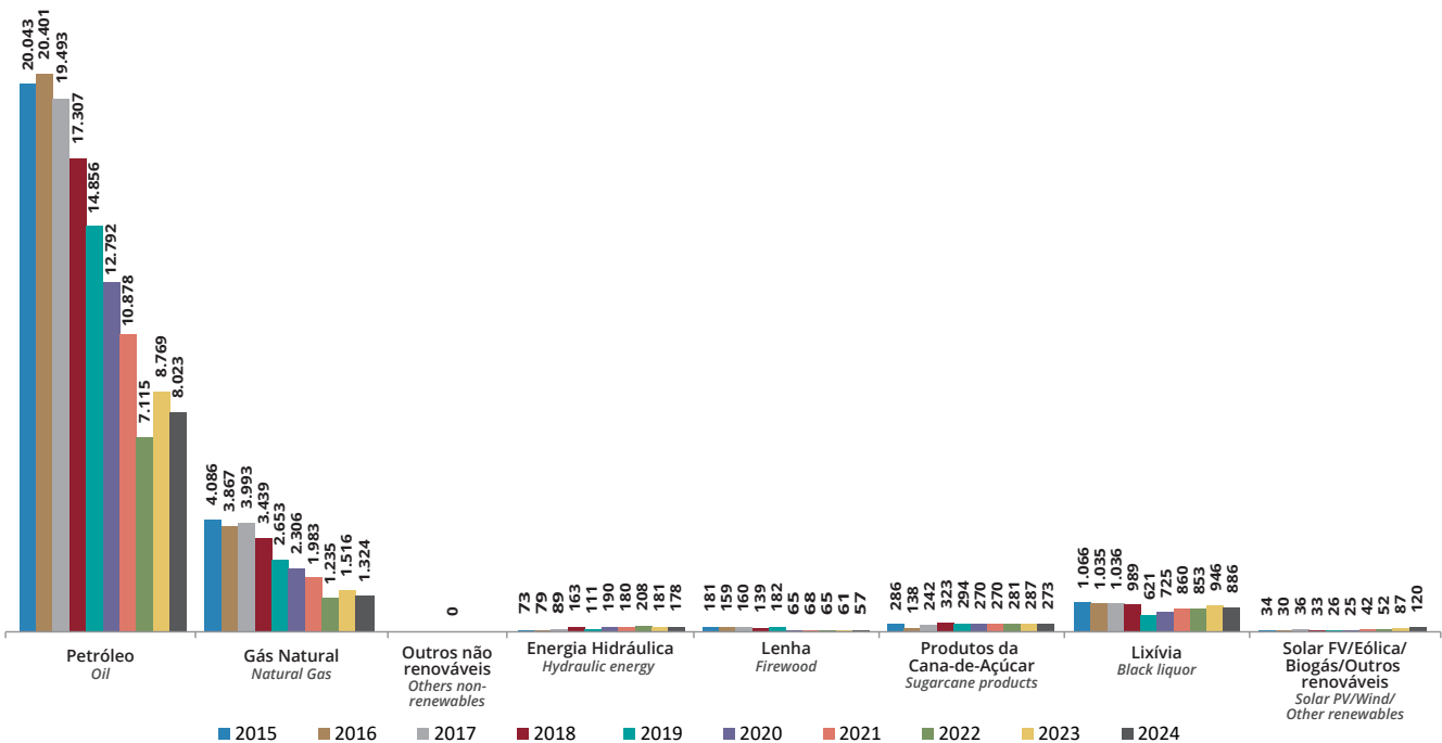
Graph 3.1.3 - Evolution of Energetic Production in Espírito Santo by Source - Values in thousand toe
