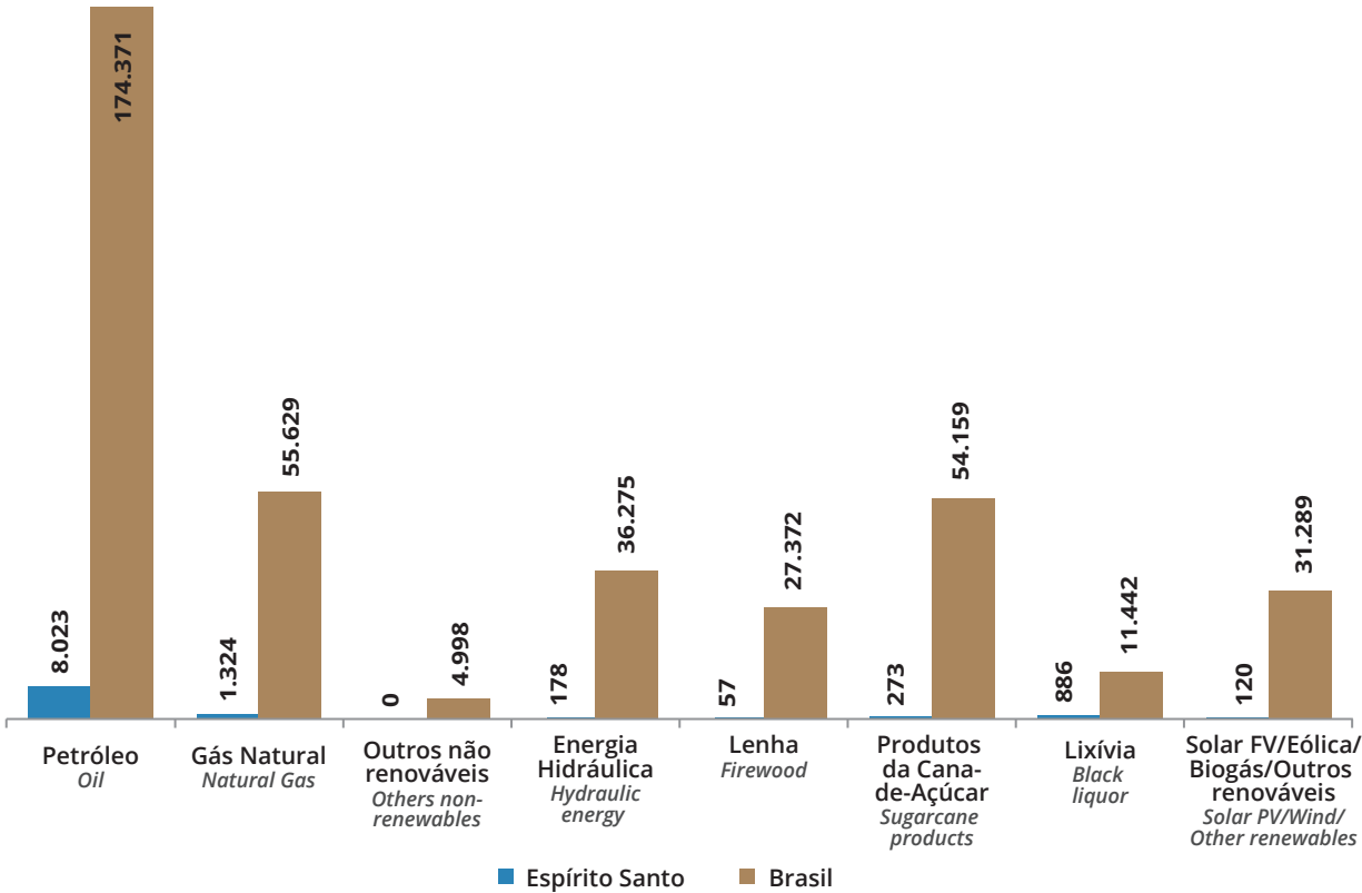
Graph 3.1.2 - Comparison of Energy Production Espírito Santo X Brazil - 2024 - Values in thousand toe
